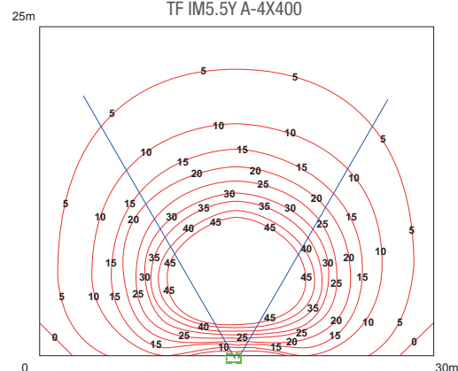
ISOLUX DIAGRAMS TF IM5.5Y A-4X400
