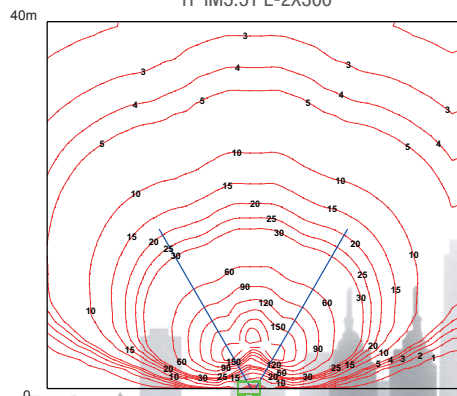
ISOLUX DIAGRAMS TF IM5.5Y L-2X300
